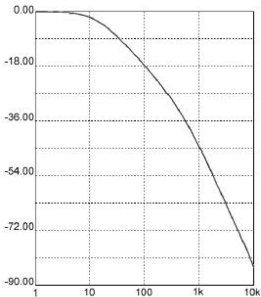
Jitter Attenuation dB vs. Frequency. E1 G.703 Input to AES output
